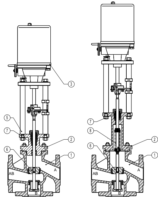
V-Rings Packing valve
