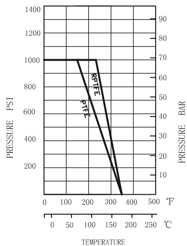
PRESSURE-TEMPERATURE RATING
