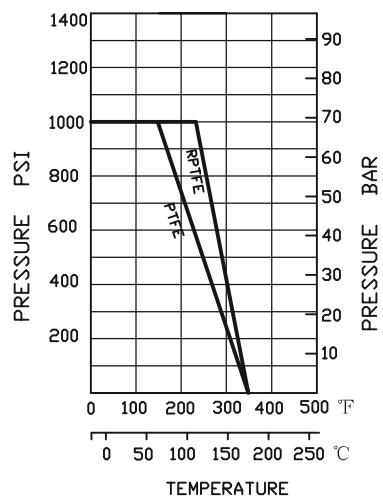
PRESSURE-TEMPERATURE RATING
