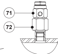
VB21M - Vacuum breaker
